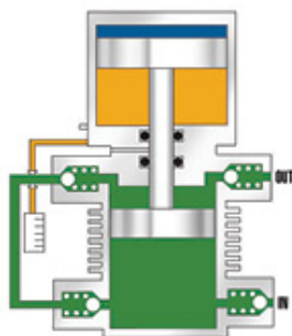
Model AGT Two Stage, Cooling Fins
