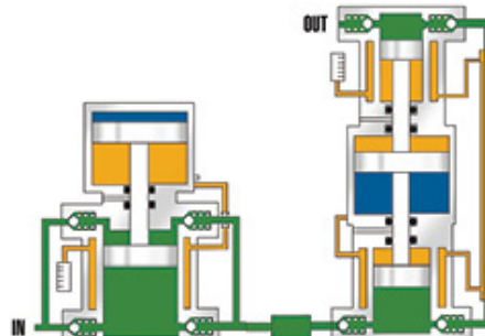
Model AGD-4 feeding into Model AGT-x/x
