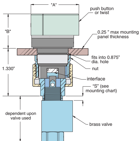
PB-22-X Adapter
