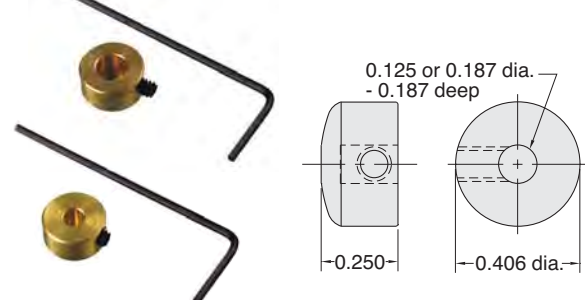
Round Solid Brass 13/32" dia. Push Button
