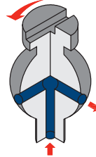
3-way Diverting
