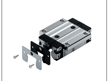
One and two-piece FKM seal 1)
