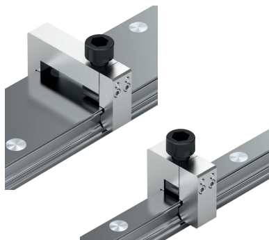
Two-piece mounting device for steel caps
