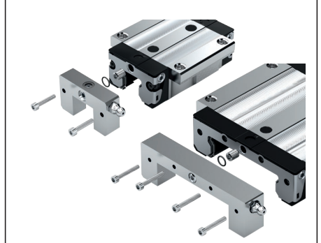
Lubrication plate 1)
