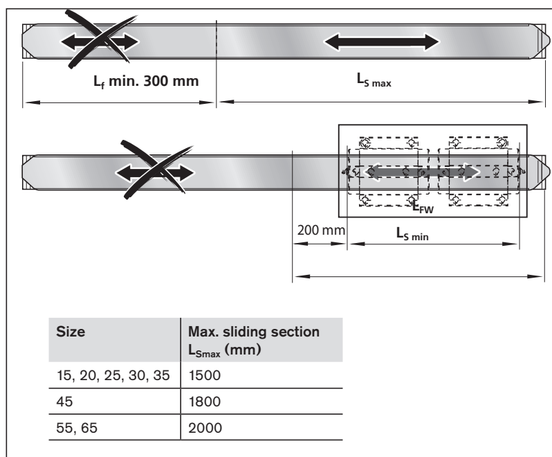
Fig. 47: Calculating the length of the sliding fit
