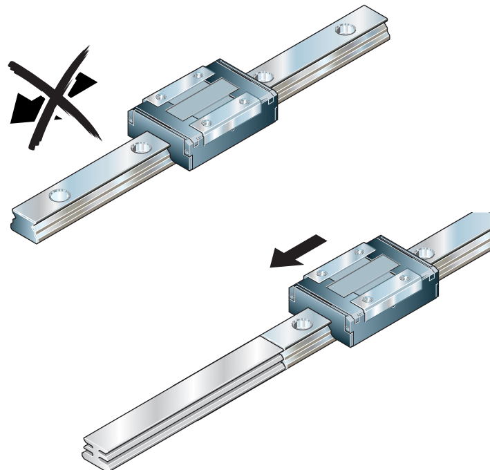
Fig. 69: Removing the MKS runner blocks
