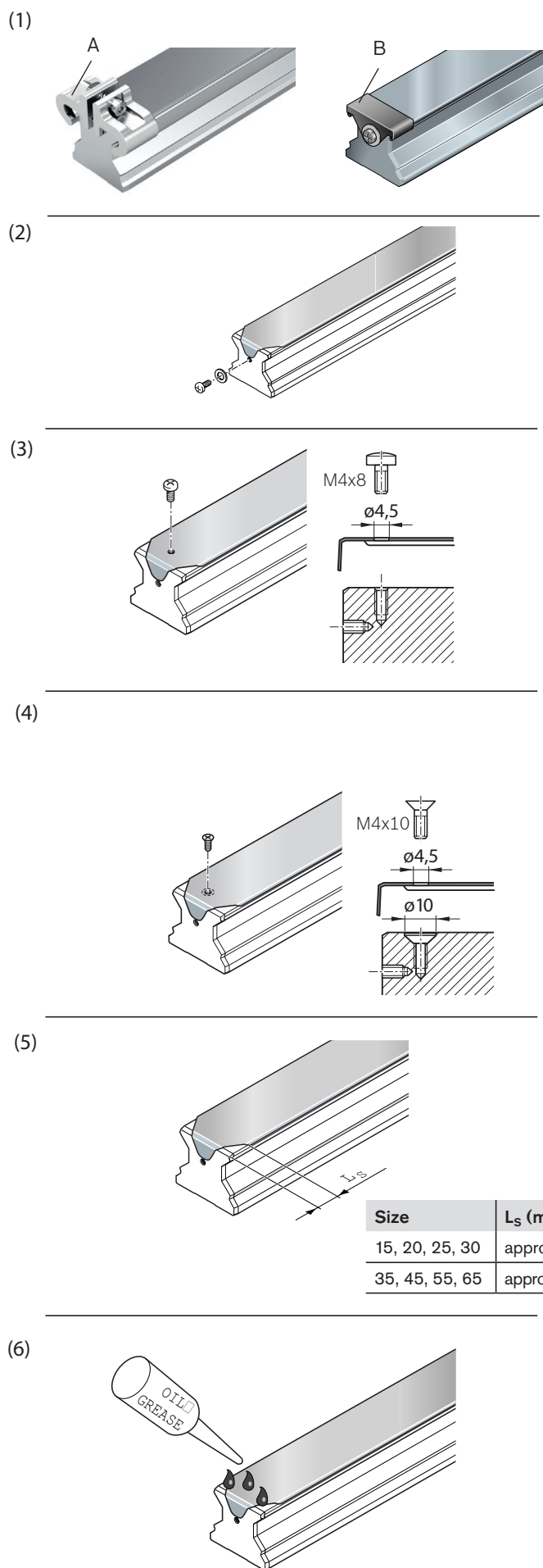
Fig. 51: Securing the Rail Seal
