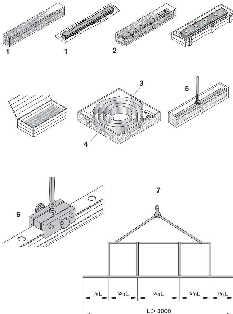
Fig. 4: Weight and delivery of guide rails
