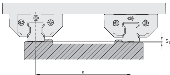
Fig. 19: Checking the vertical offset of the guide rails
